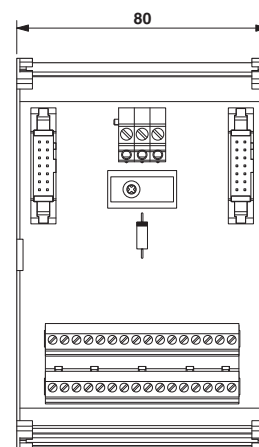
Dimensioned drawing
