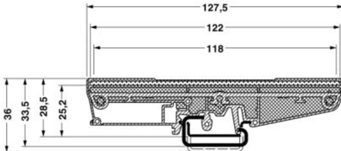
Dimensioned drawing
