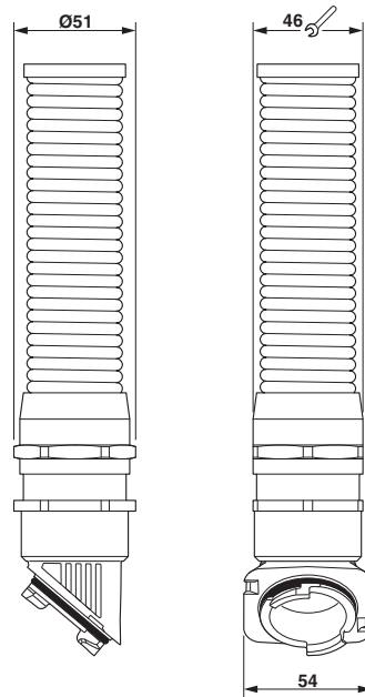
Dimensional drawing
