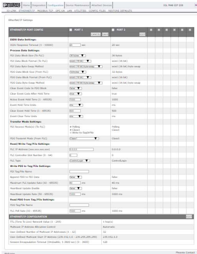
Figure 5-13 “EtherNet/IP Settings” page
