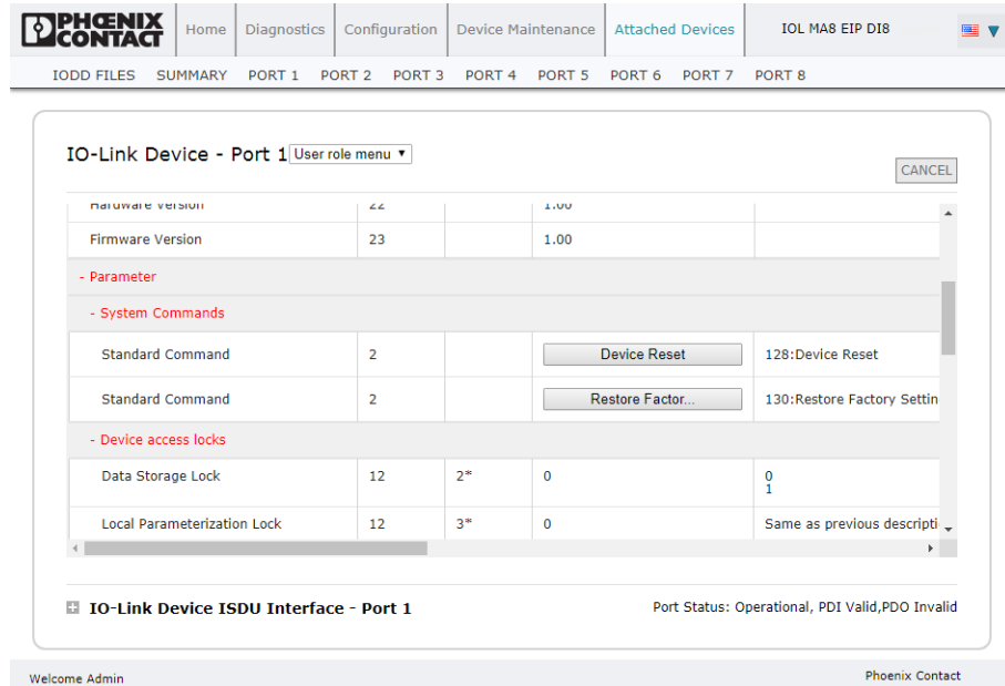
Figure 5-43 Reset Factory IO-Link defaults
