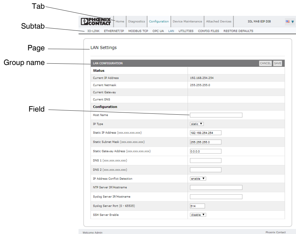
Figure 4-1 GUI terminology
