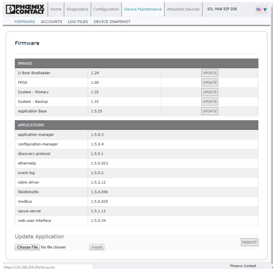
Figure 5-27 “Firmware” page
