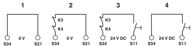
Figure 15 Start and feedback circuit connection variants
