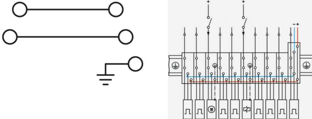
Circuit diagram
