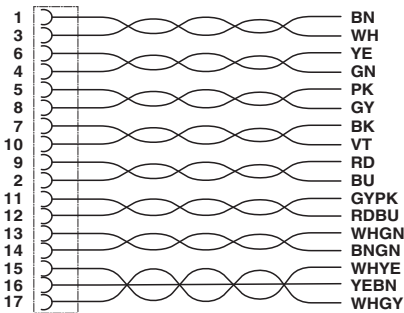
Contact assignment of the M12 socket
