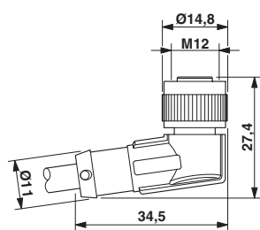
Dimensioned drawing
