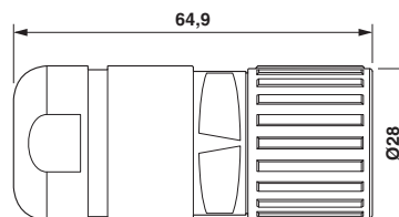
Dimensional drawing
