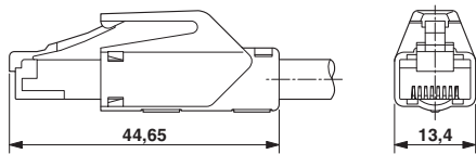
Dimensioned drawing
