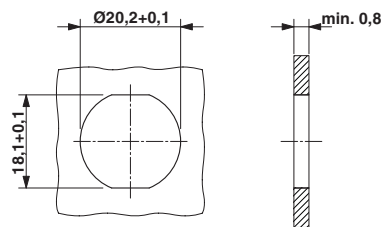
Dimensioned drawing
