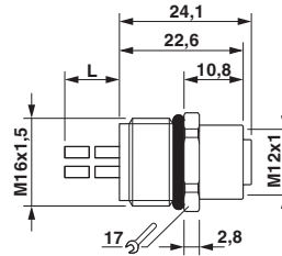
Dimensioned drawing
