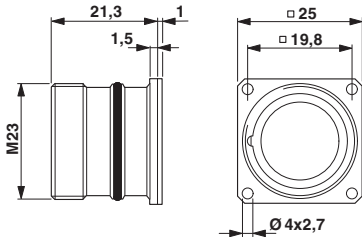
Dimensioned drawing
