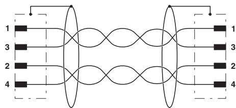
Contact assignment of the M12 plugs
