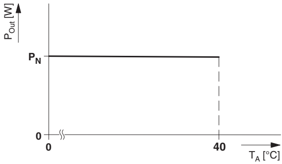
Figure 25 Temperature-dependent derating
