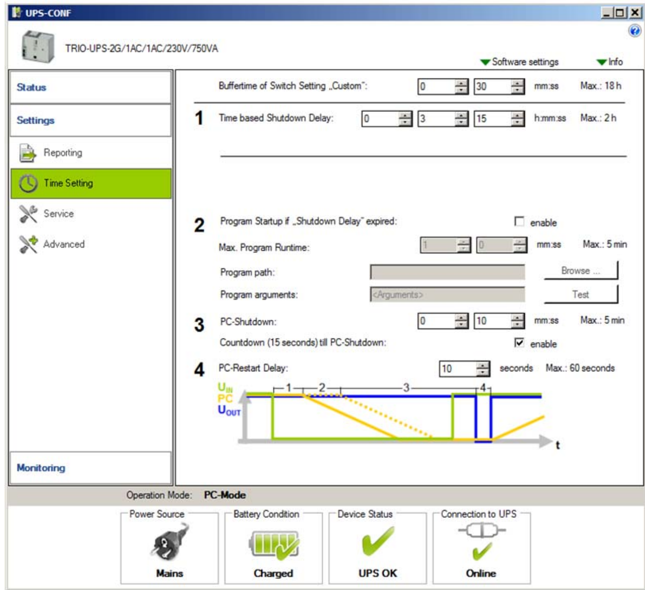
Figure 19 Time setting
