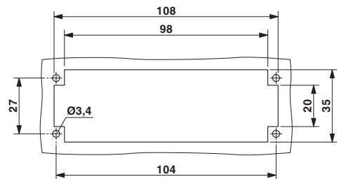
Panel cutout
