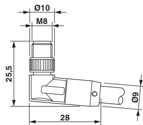
Dimensional drawing
