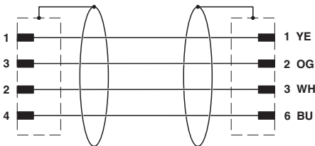
Contact assignment of the M8 and RJ45 plug
