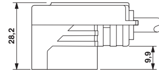
Valve connector, type B, side view
