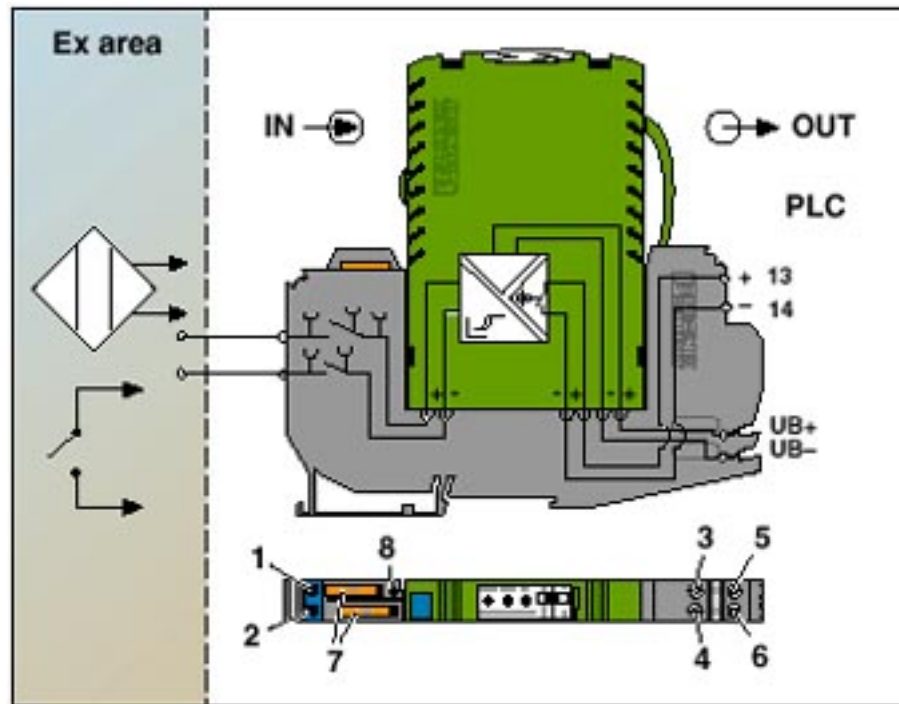
Circuit diagram
