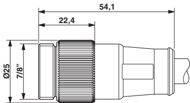
7/8" connector, straight
