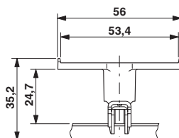
Dimensional drawing
