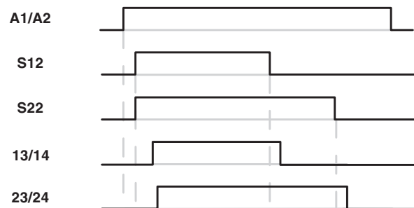
Figure 4 Time diagram
