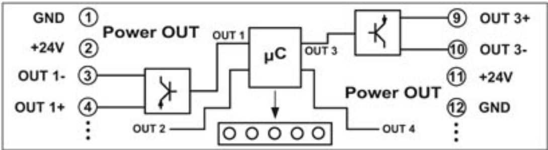
Block diagram
