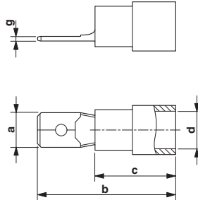
Dimensioned drawing
