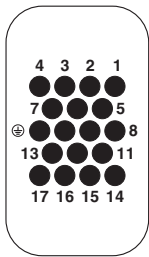
Connector pin assignment, connection side
