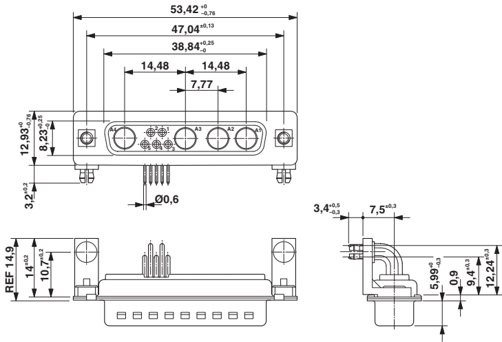
Dimensioned drawing
