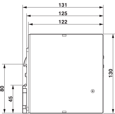
Figure 4 Device dimensions (dimensions in mm)
