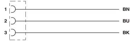
Contact assignment of the DEUTSCH DT06-3S
