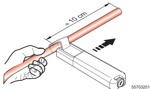
Figure 30 Stripping the outer cable sheath
