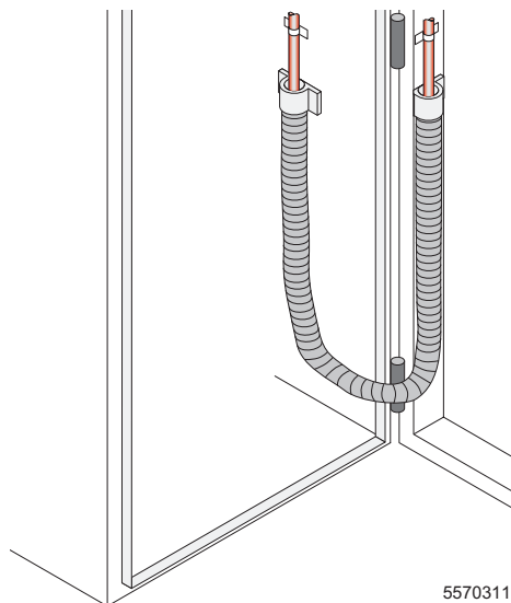
Figure 12 Spiral tube
