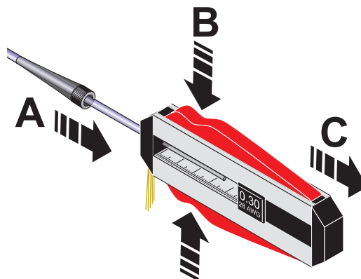
Figure 37 Removing the coating
