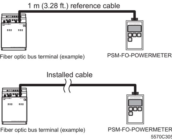
Figure 50 Power measurement of fiber optic cables
