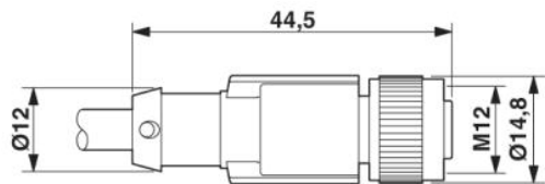
Dimensioned drawing
