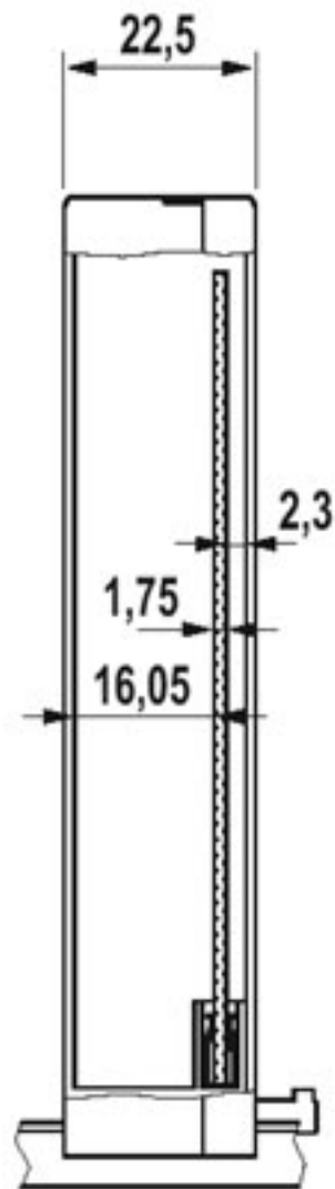
Dimensioned drawing
