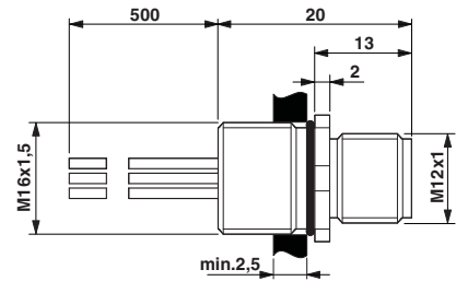
M12 flush-type connector
