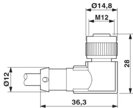
Dimensioned drawing
