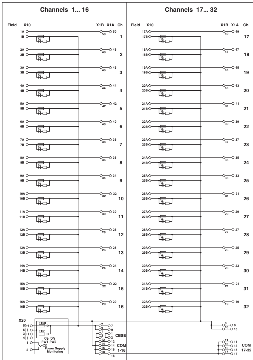
Circuit diagram
