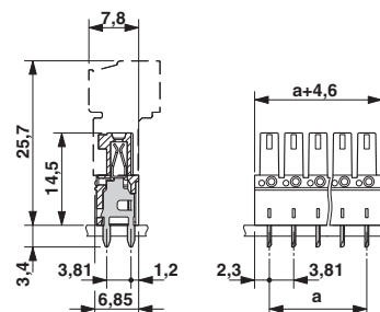
Dimensioned drawing
