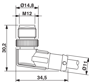
Dimensioned drawing
