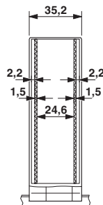
Dimensioned drawing
