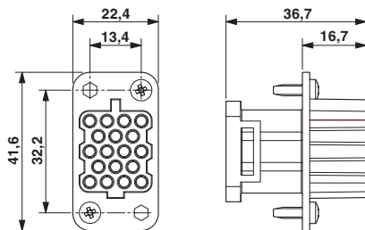
HC-COM-17-EBUC dimensional drawing
