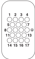
Connector pin assignment, connection side
