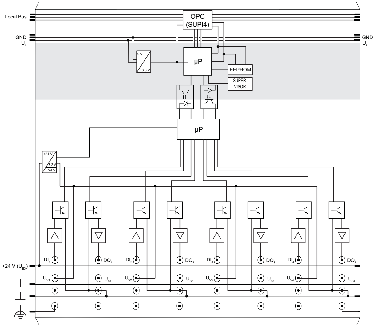
Figure 1 Internal wiring of the terminal points
