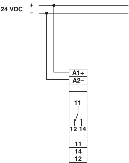
Figure 1 Connection without control contact
