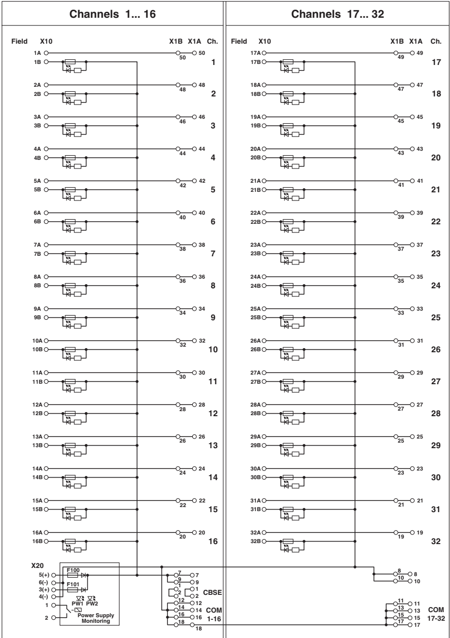
Circuit diagram
