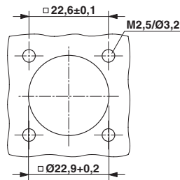
Dimensioned drawing
