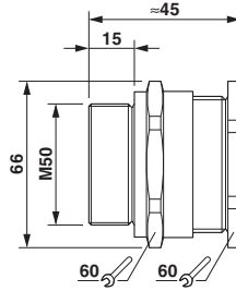
Dimensional drawing
