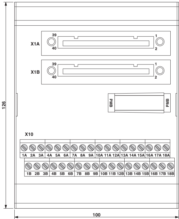
Dimensional drawing
