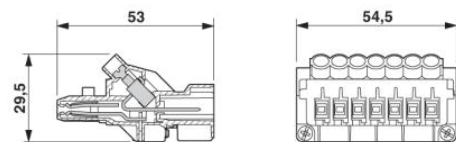
Dimensioned drawing
