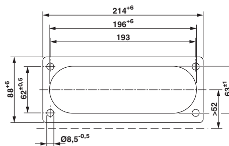
Wall cutout drawing
