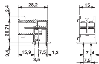
Dimensioned drawing
