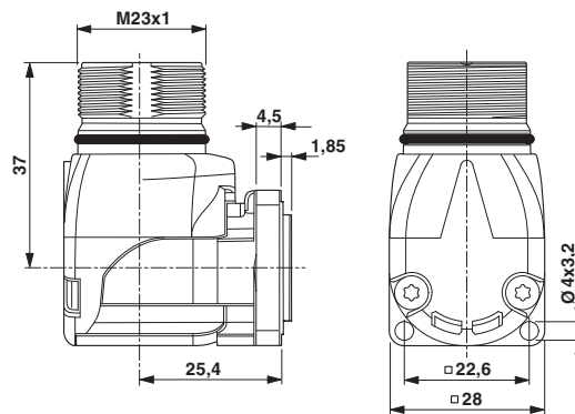
Dimensioned drawing
