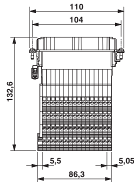
Dimensioned drawing
