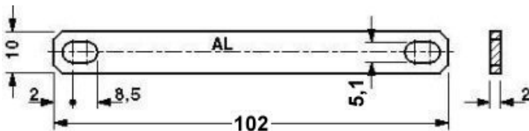
Dimensioned drawing
